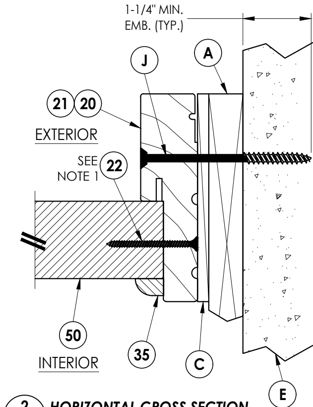
2/4 HORIZONTAL CROSS SECTION Shown w/1X sub-buck
