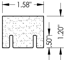
45 BOTTOM RAIL Cellular PVC
