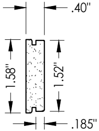
43 LATCH & HINGE STILE Cellular PVC
