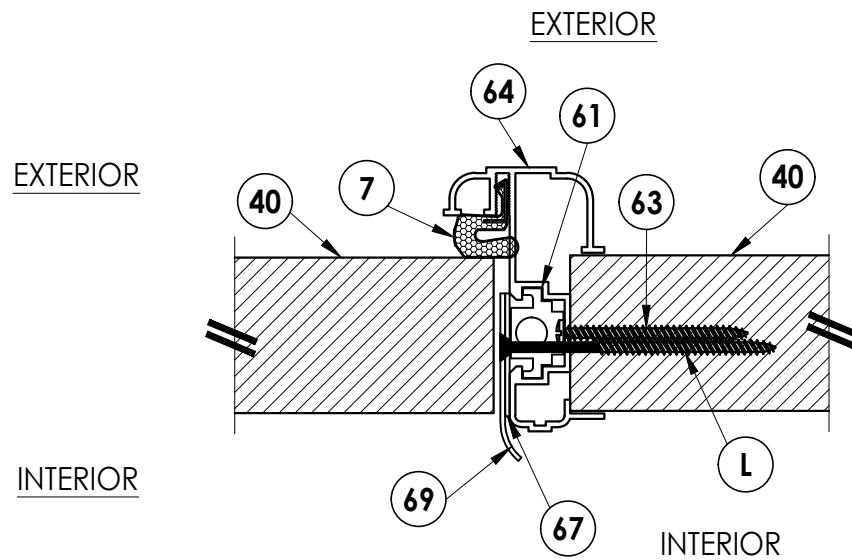
3/4 HORIZONTAL CROSS SECTION
